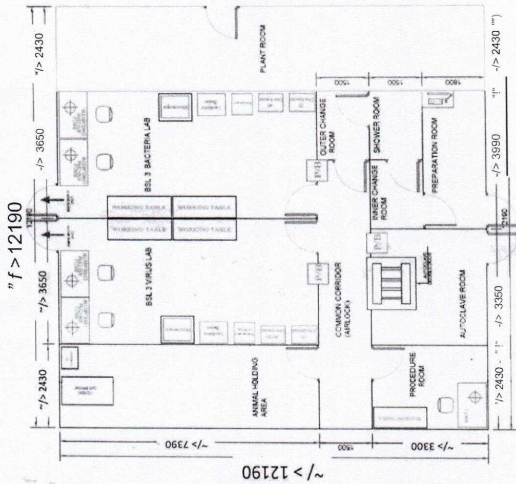
Reference Layout for Modular BSL3
