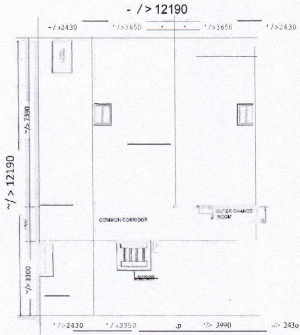
Reference Layout for Modular BSL3
