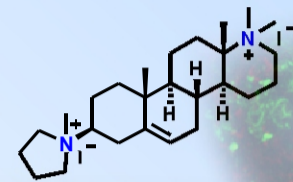
Chandonium iodide (Neuromuscular blocker)
