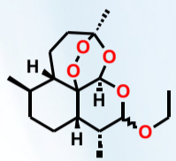
\alpha - \beta Arteether (antimalarial)
